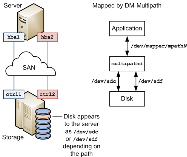
Figure 19.2 DM-Multipath Mapping of Two Paths to a Disk over a SAN
